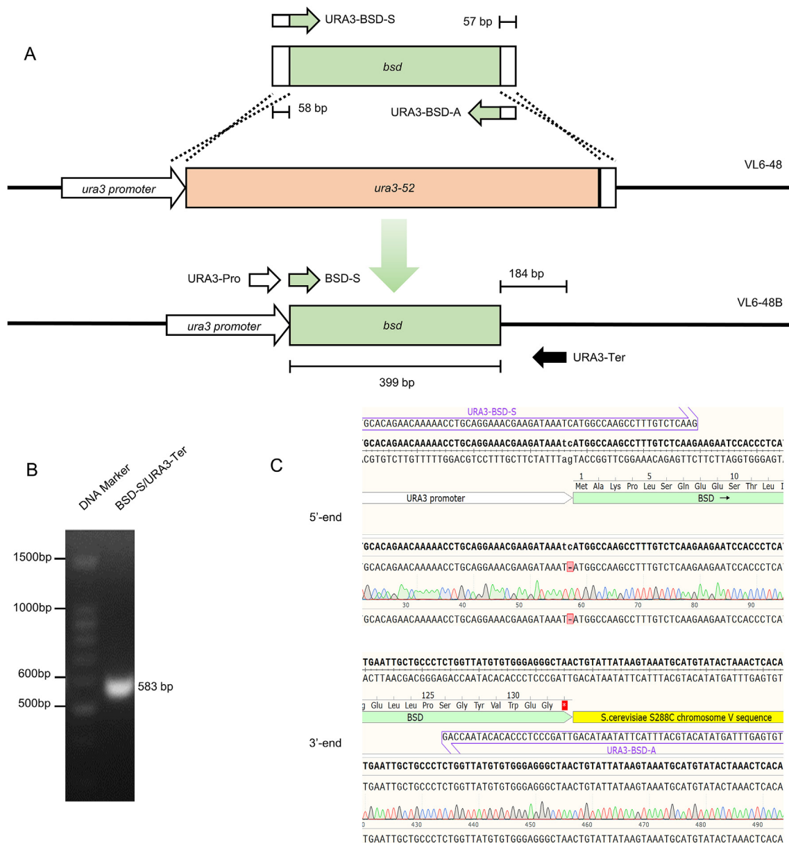
Fig. 1. Development of the ura3-52 -defective strain VL6-48B. A A diagram of the ura3-52 locus in VL6-48 and primer pairs for amplifying the bsd gene ( URA3-BSD-S/A ), genotyping ( BSD-S/URA3-Ter ), and sequencing ( URA3-Pro ) of the transgene. The PCR amplicon of bsd contains 58- and 57-bp homologous sequences surrounding the ura3-52 open reading frame (ORF) at its 5'- and 3'-termini. The primers for genotyping targeted the start codon and 184 bp downstream of the ura3-52 ORF. B The genomic content of transformed yeast was extracted and served as the template for genotyping PCR. The amplicon was then subjected to gel electrophoresis, and a 583-bp band was seen by ethidium bromide staining. C The genomic content of transformed yeast was extracted and subjected to sequencing using the primer URA3-Pro . The sequenced region consists of bsd at the center region and the ura3 surrounding sequence at the 5'- and 3'-ends.
