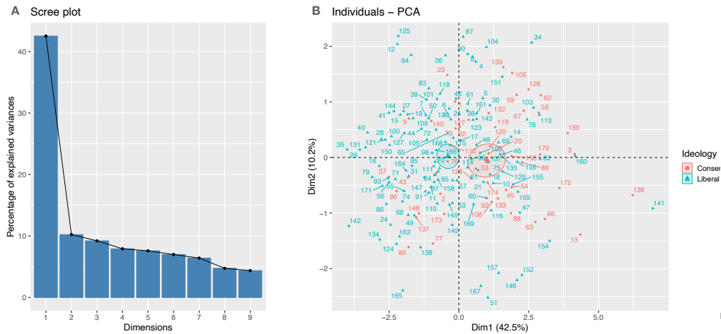
Fig. 2. Panel A shows a scree plot describing the percentage of variation explained by the principal components for the political ideology scores across all nine fMRI tasks. Panel B provides a biplot representing the principal component scores for all participants in the study. Points are colored according to political ideology. Ellipses represent the 95% confidence interval of principal component scores for each ideology.
