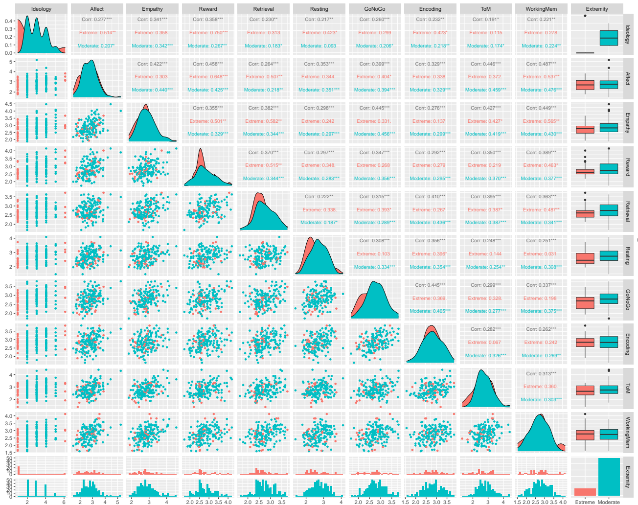
Fig. 1. Pairwise associations of FC scores and their associations with Political Ideology. Scatterplots show the relationship between the predicted political ideology score from each FC task once applied to BrainNetCNN and the true ideology. Points are colored according to extremity of true ideology: red points show extreme views (very liberal or very conservative) and blue points show moderate views (liberal, somewhat liberal, moderate, somewhat conservative, conservative). Correlations are provided for all ideology values (in black), moderate only (in blue), and extreme values (in red). Correlation values with *** are statistically significant with p -value < 0.001 and those with ** are statistically significant with p -value < 0.01 and those with * are significant at p -value < 0.05 .
