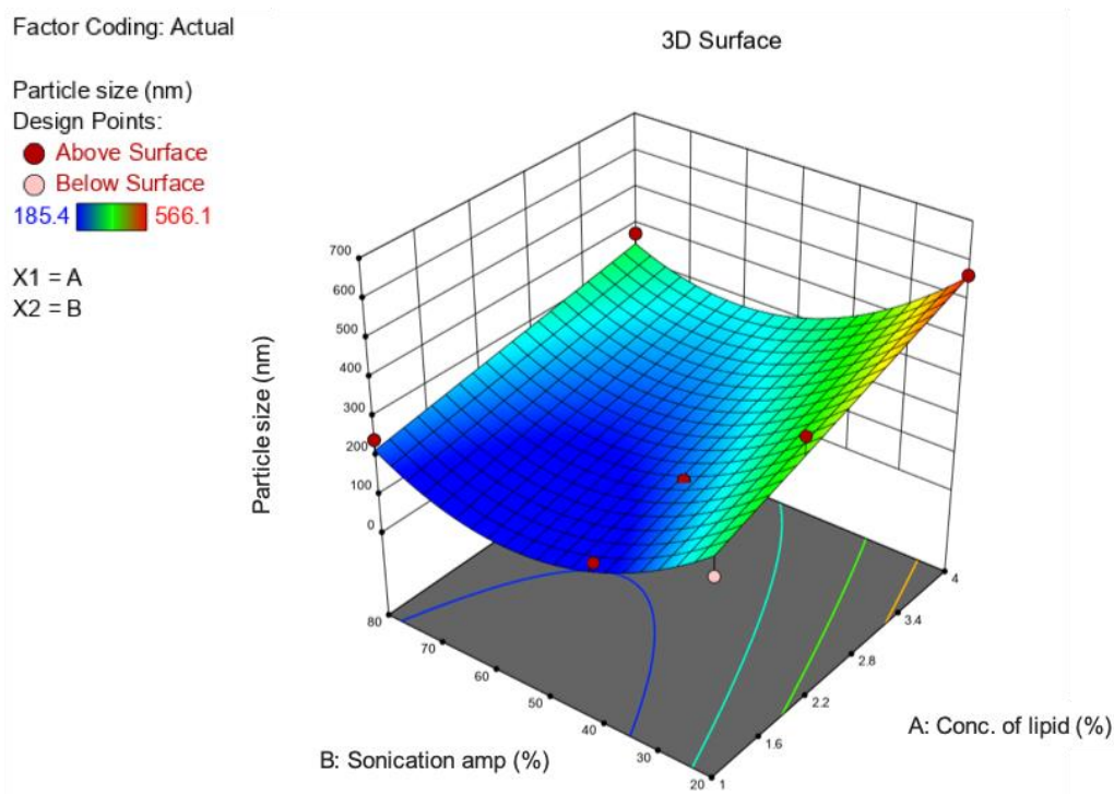
Figure 4. The 3D response surface plot showing the effects of the lipid concentration (A) and sonication amplitude (B) on the particle size of berberine-loaded phytantriol-based LCNs.
