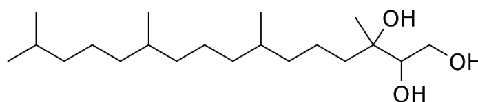
Figure 2. Structure of phytantriol.
