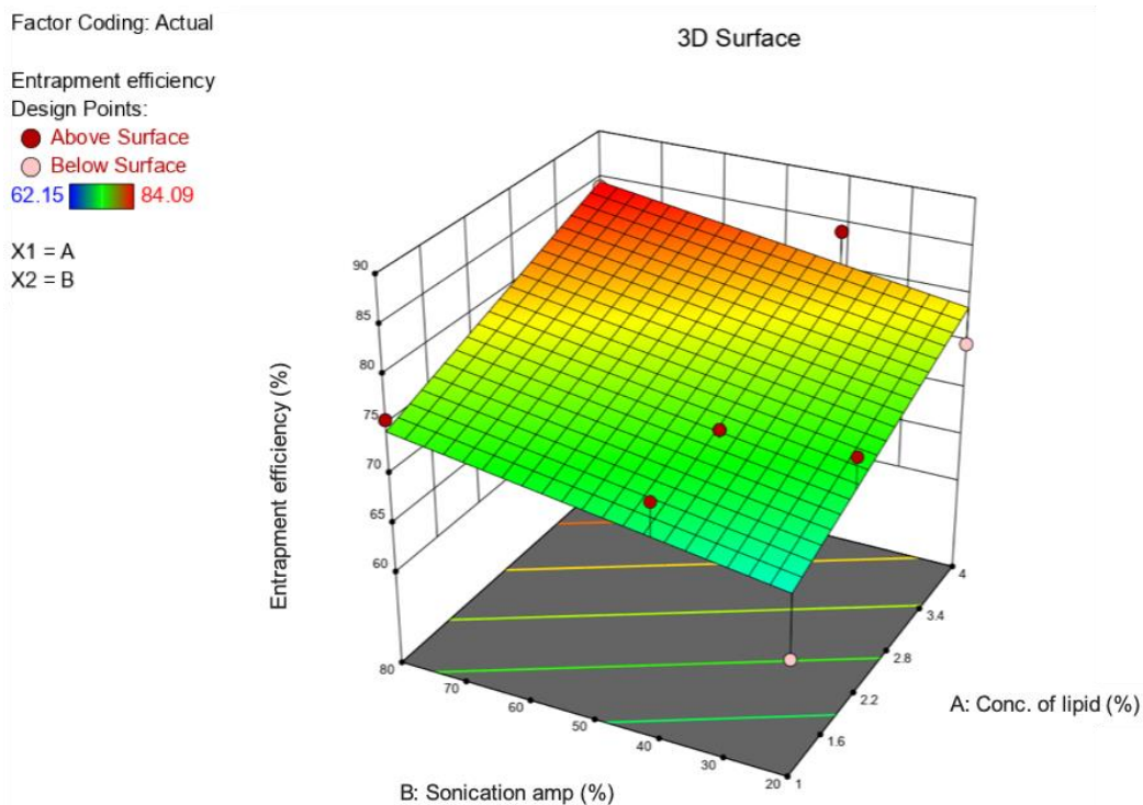
Figure 5. The 3D response surface plot showing the effects of the lipid concentration (A) and sonication amplitude (B) on the entrapment efficiency of berberine-loaded phytantriol-based LCNs.
