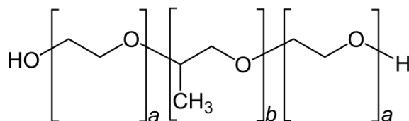
Figure 3. General structure of poloxamer (where poloxamer 407 has block lengths of a = 101 and b = 56 ).
